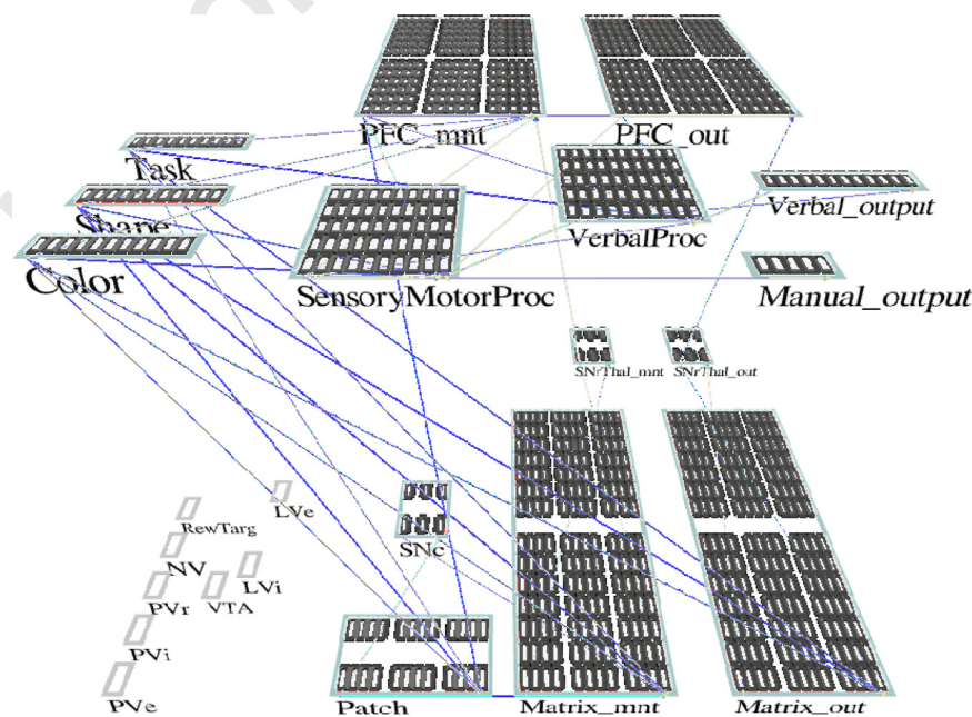
Fig. 3. Model Architecture. Each small rectangle is a single unit. Lines to the bottom right of a layer are incoming connections, while those from the left are outgoing connections. The general flow of information processing proceeds from left to right, from Color, Shape, and Task inputs, through the two Processing (hidden) layers, to the Verbal and Manual outputs. The PFC layer holds information in active states from previous trials and that information modulates processing in the two hidden layers. The PFC layer is composed of stripes, each of which is “gated” to maintain information based on the result of learning in the Matrix (striatum). This learning is in turn based on a predicted reward, calculated in the PVLV module (lower left), which is shown without units and connections to make other connections visible. The PBWM framework and the PVLV system are described in detail elsewhere; see text for references.
